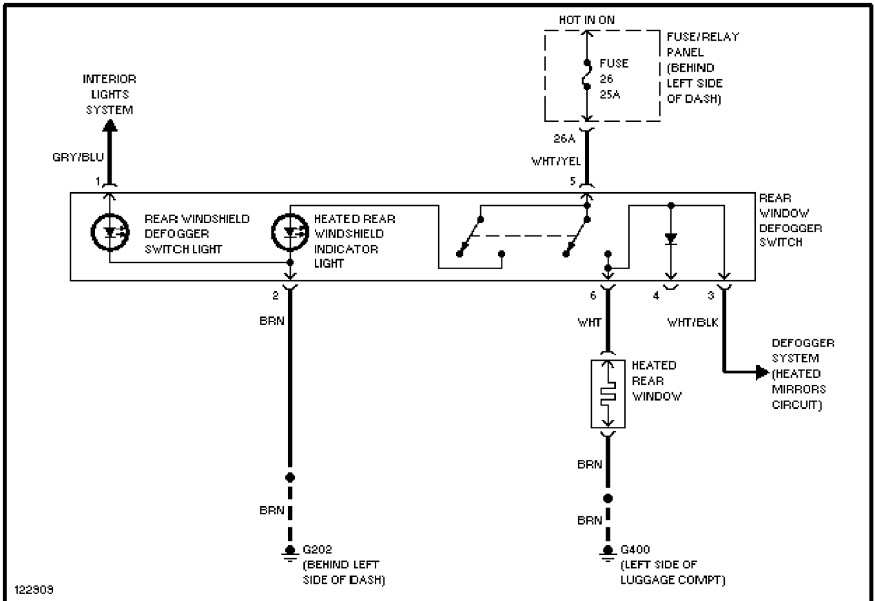
Rear Defogger Circuit
