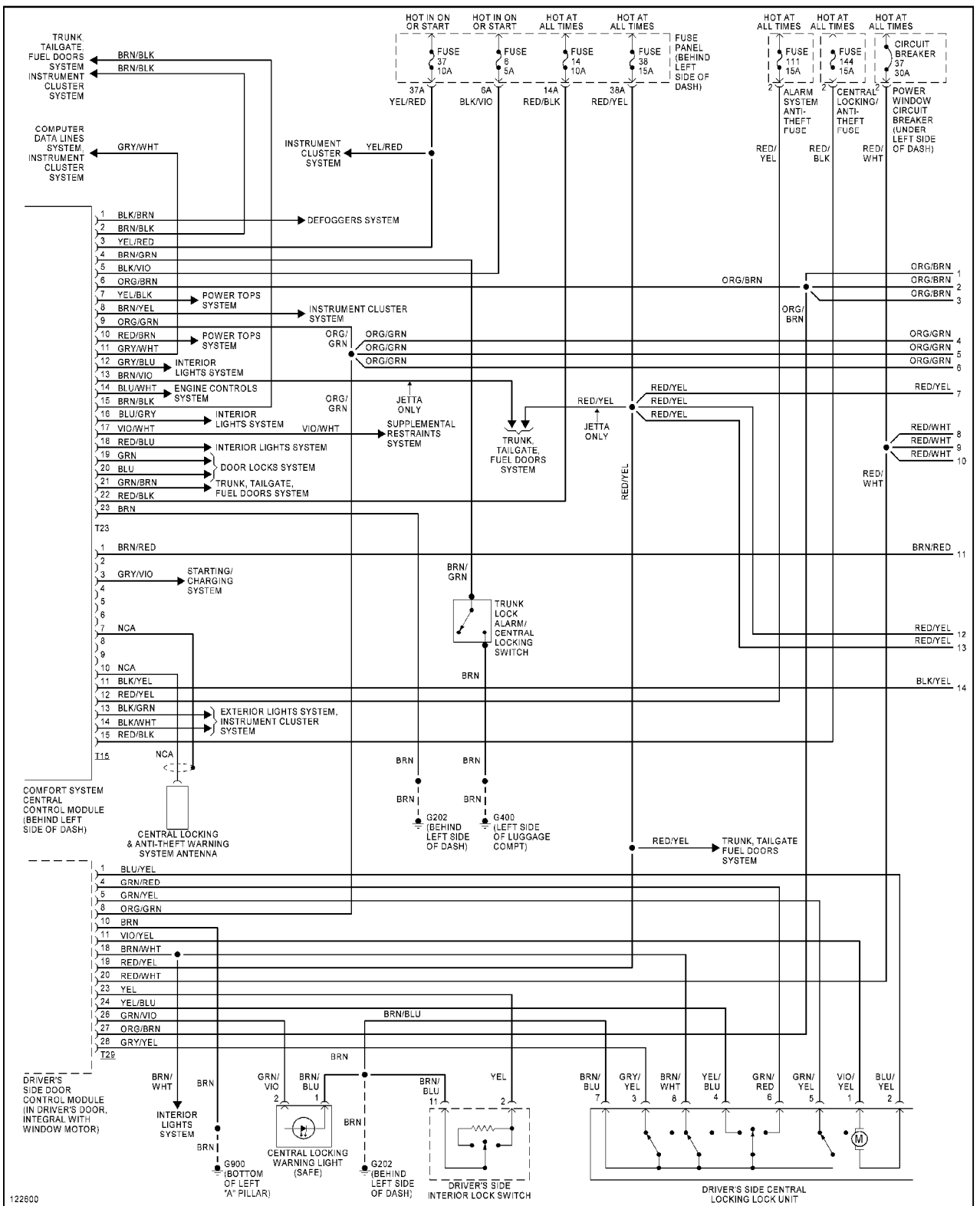
Anti-theft Circuit, W/ Power Windows (1 of 2)
