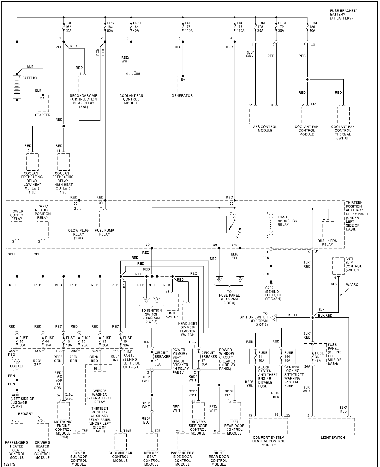
Power Distribution Circuit (1 of 3)
