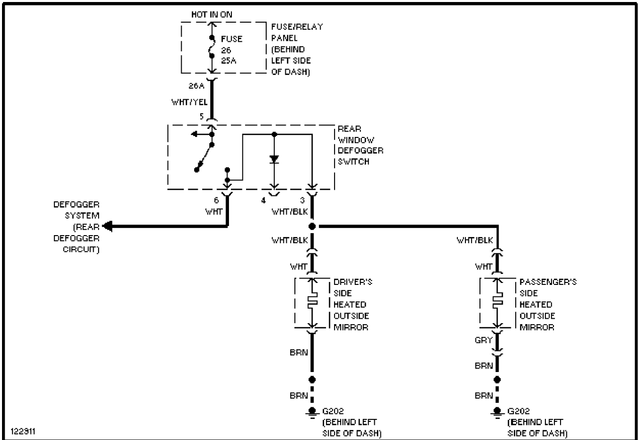
Heated Mirrors Circuit, W/O Power Windows
