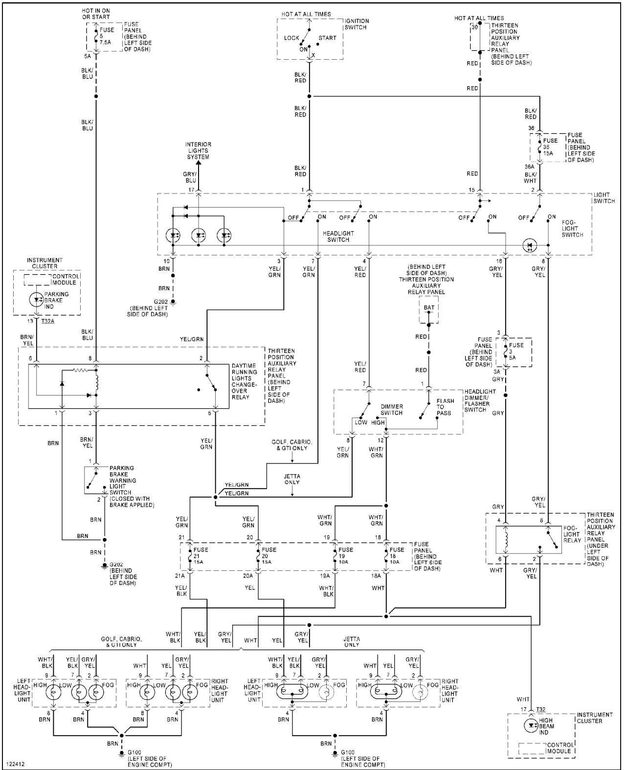
Headlight Circuit
