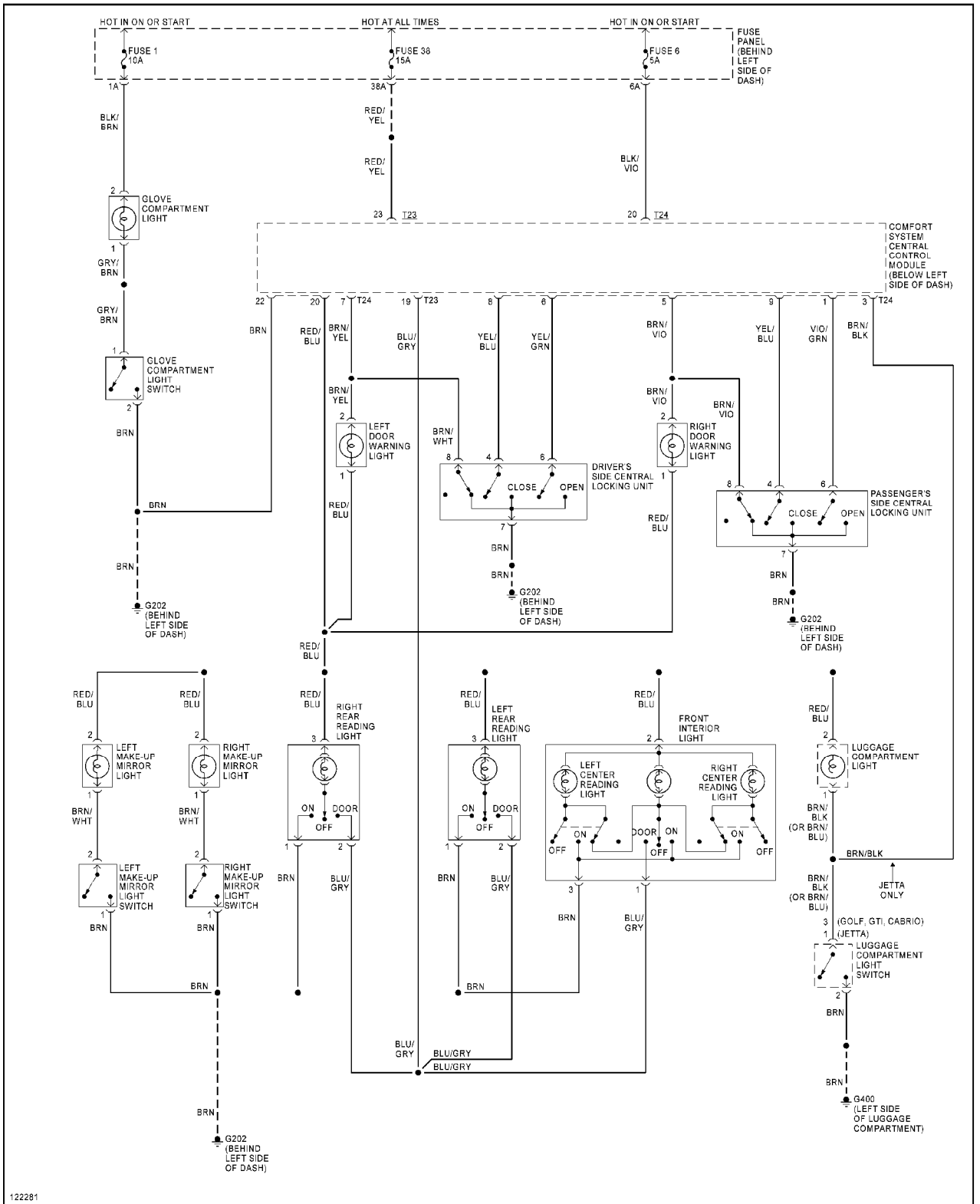
Courtesy Lamps Circuit, W/O Power Windows
