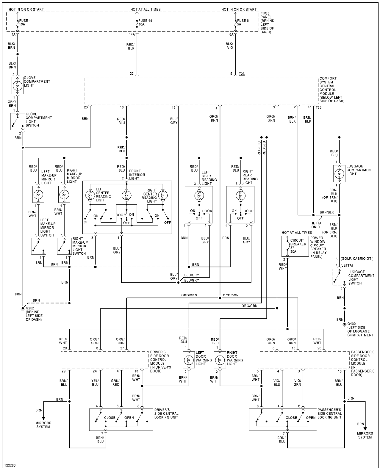
Courtesy Lamps Circuit, W/ Power Windows
