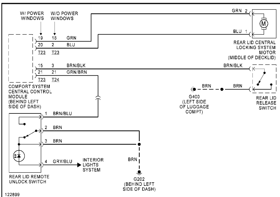
Deck Lid Release Circuit
