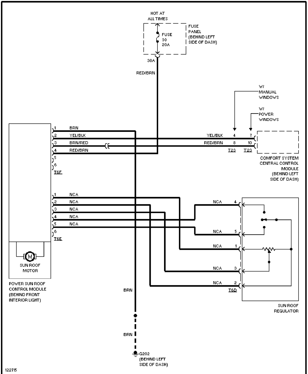
Sunroof Circuit
