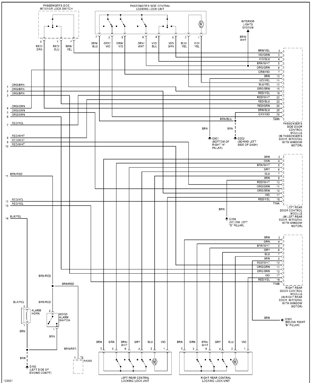
122501 Anti-theft Circuit, W/ Power Windows (2 of 2)
