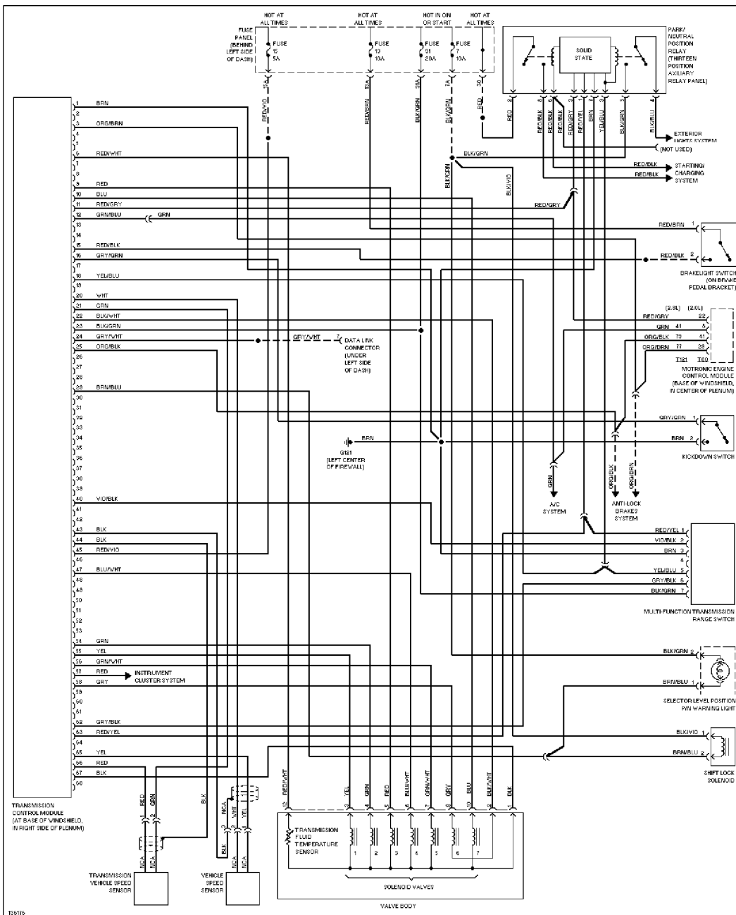
2.0L, A/T Circuit
