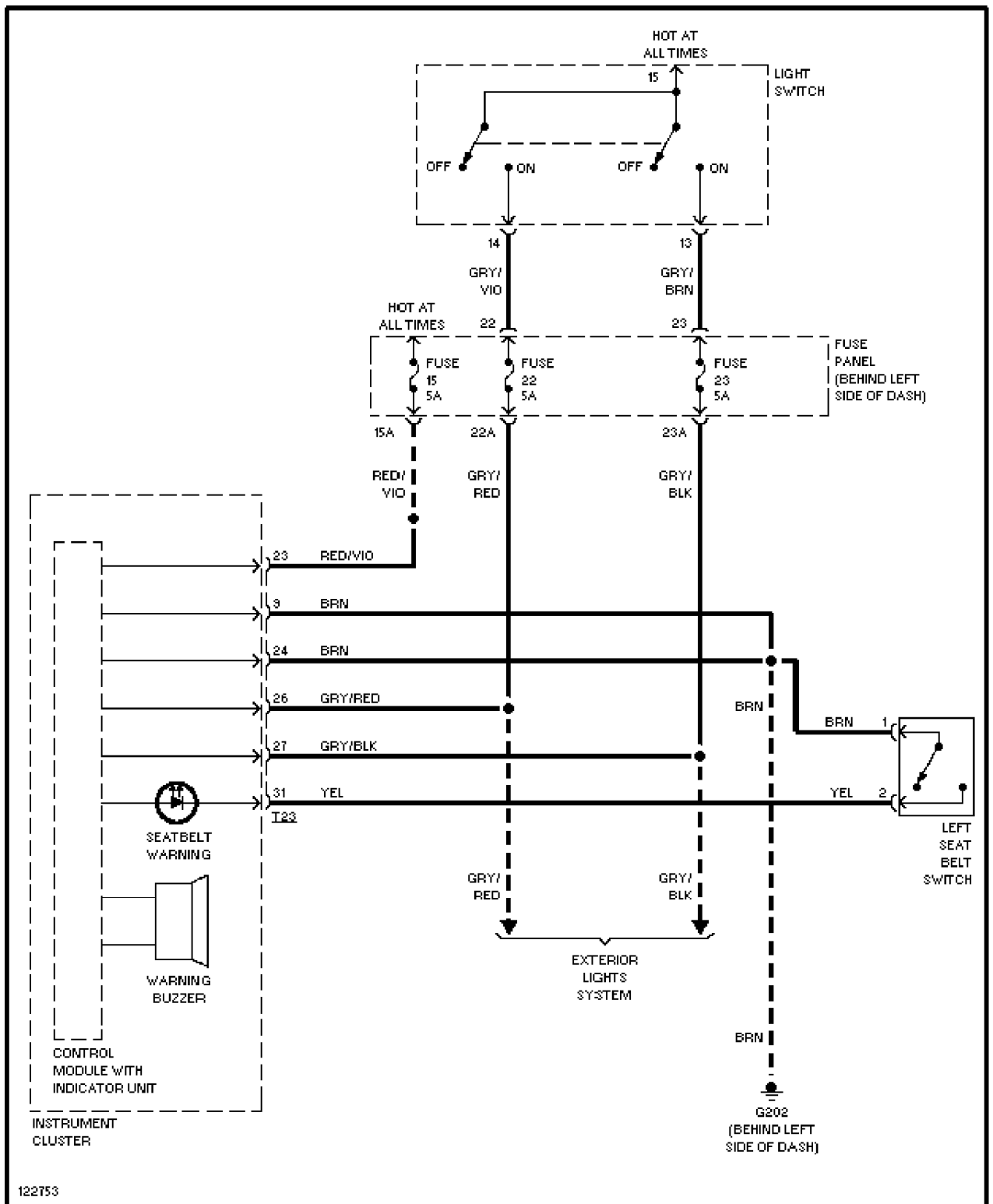
Buzzer Circuit
