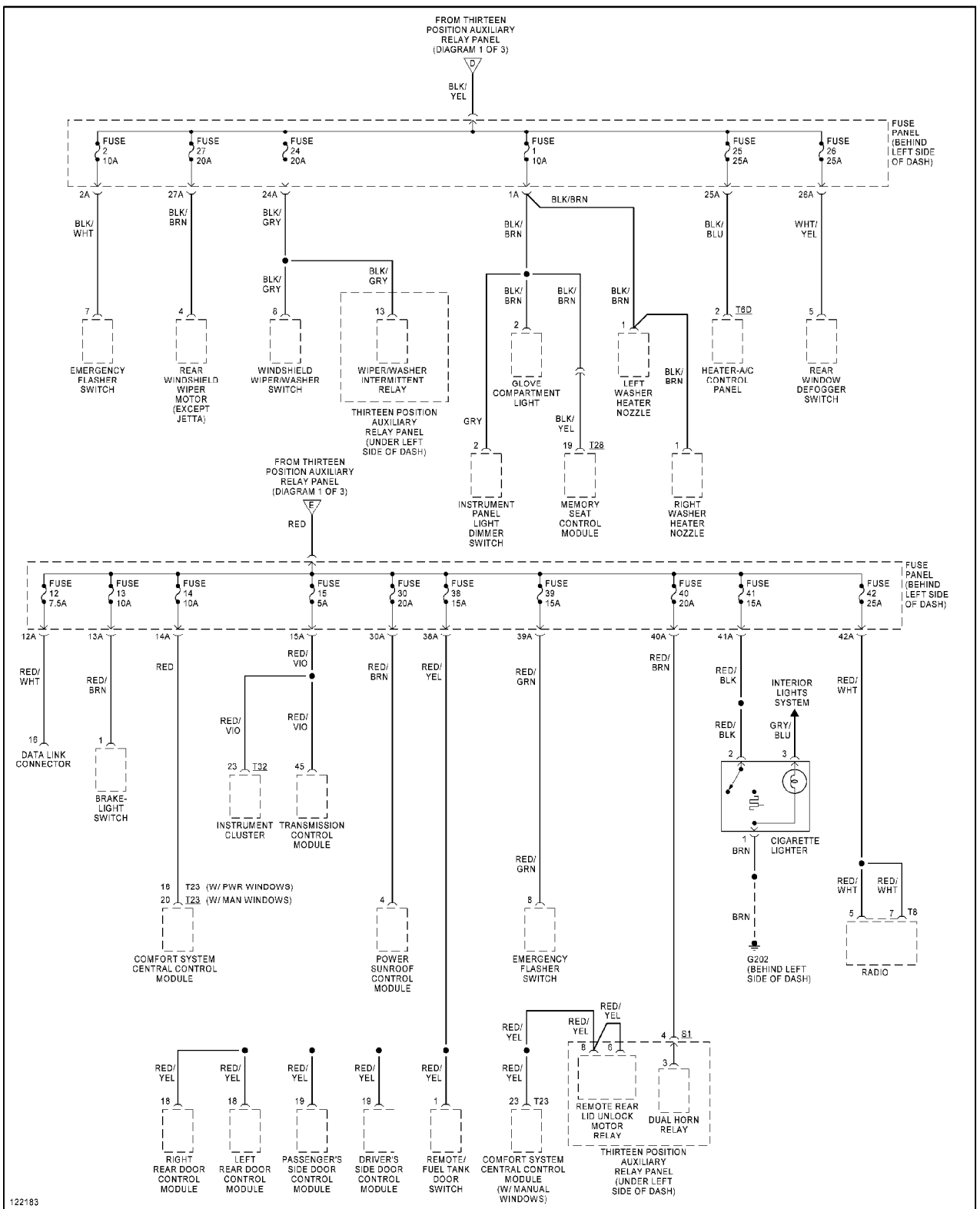
Power Distribution Circuit (3 of 3)
