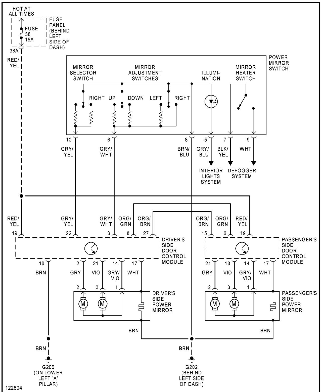
Power Mirrors Circuit
