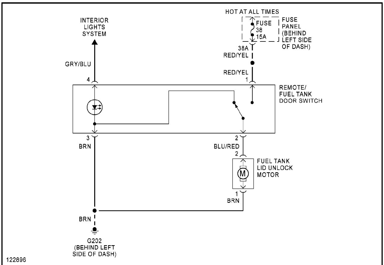
Fuel Door Release Circuit
