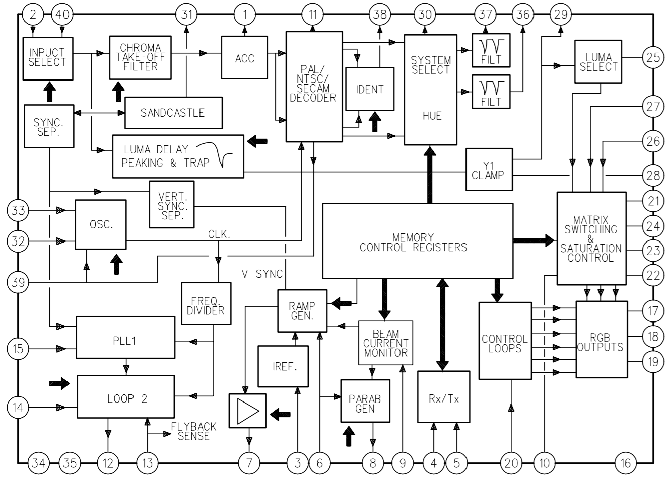
A BOARD IC301 MC4402P/MC44007P
