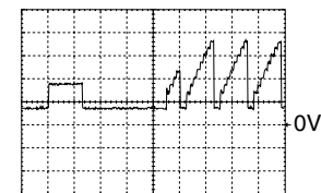
⑱ 1V/cm, 50µs/cm
