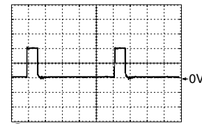
③ 5V/cm, 5µs/cm
