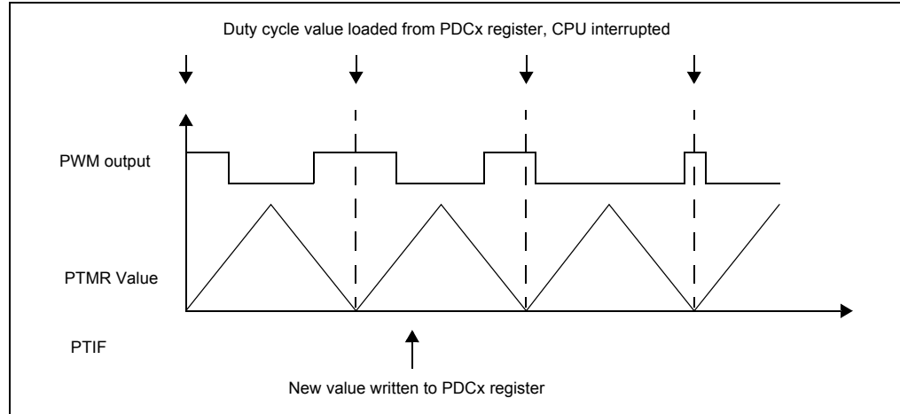
Figure 15-10: Duty Cycle Update Times in Up/Down Count Mode
