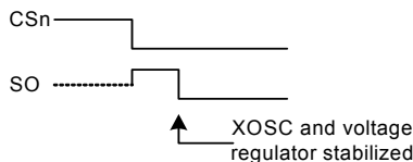
Figure 16: Power-on reset
