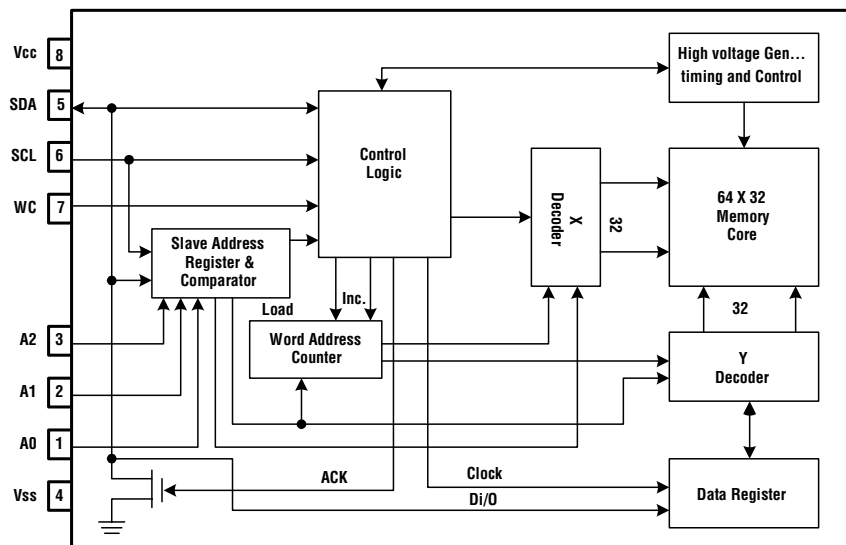
IC4 ST24C02
