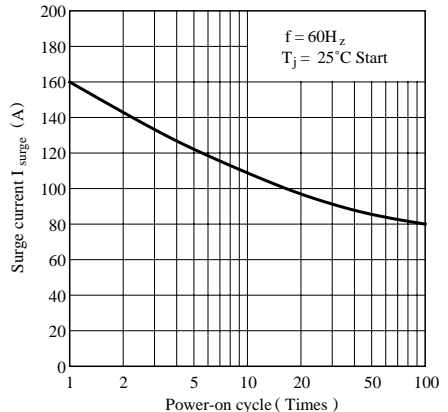
Fig.5-b Surge Current vs. Power-ON Cycle
