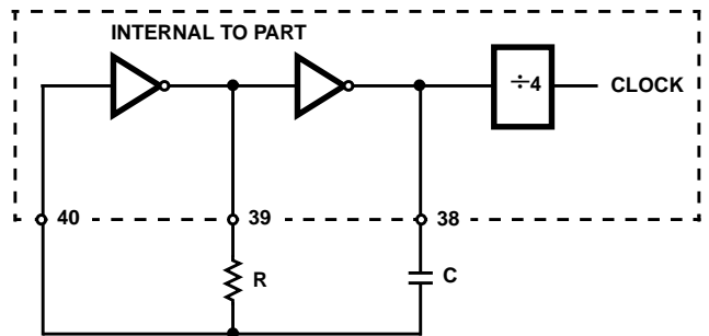
FIGURE 9B. RC OSCILLATOR FIGURE 9. CLOCK CIRCUITS
