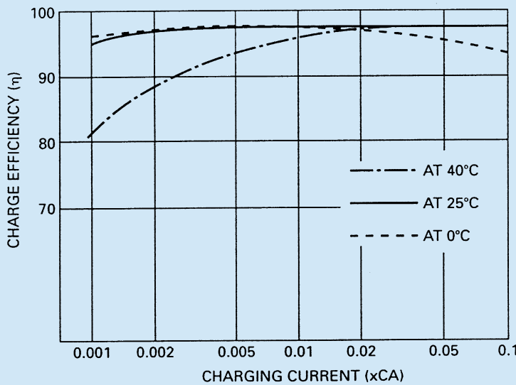
Figure 31. CHARGING EFFICIENCY
