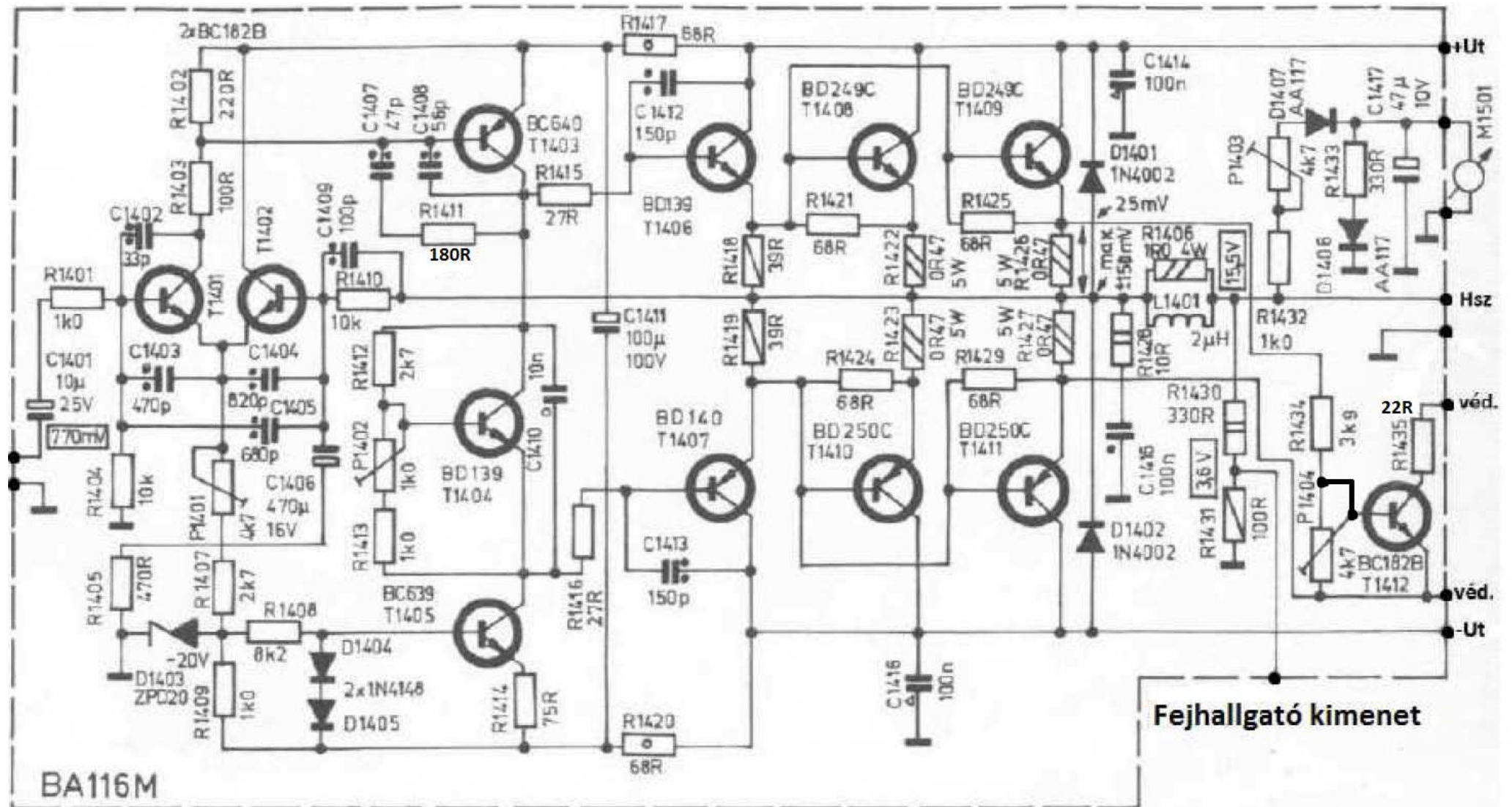
ORION SE260 amplifier Schematic
