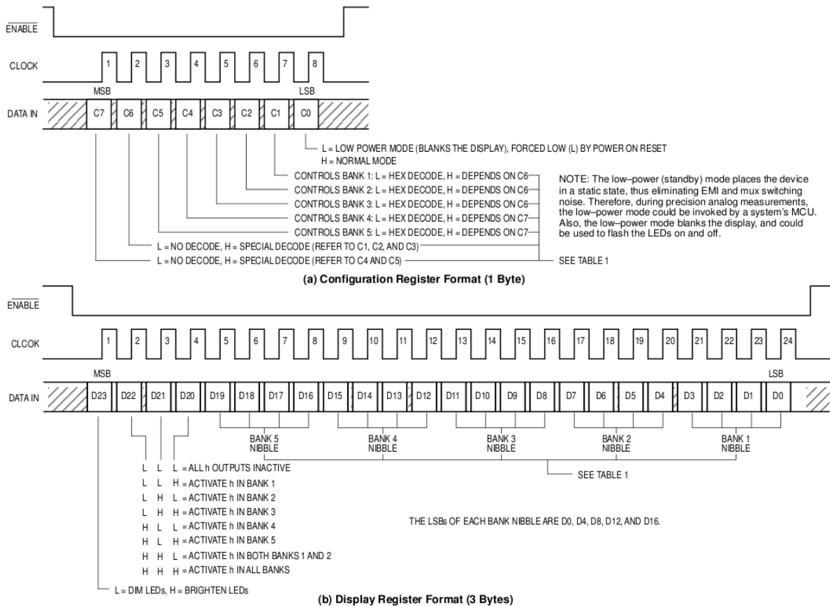
Figure 7. Timing Diagrams for Non-Cascaded Devices
