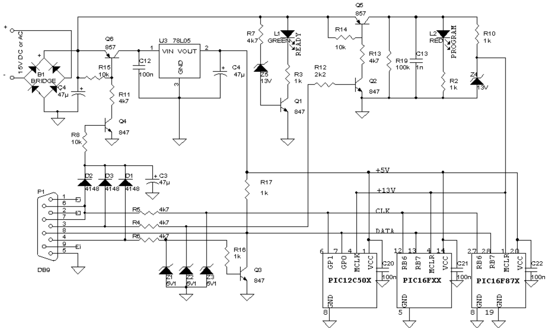
PIC16FXX / PIC16F87X / PIC12C50X PROGRAMMER
