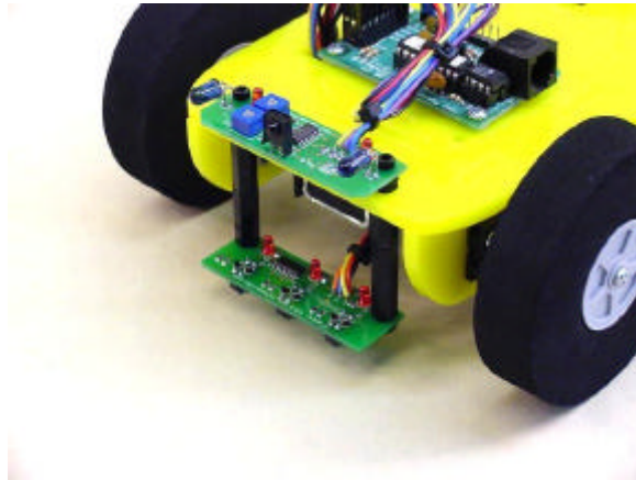
Illustration showing the Tracker mounted to a CR1 Robot.
