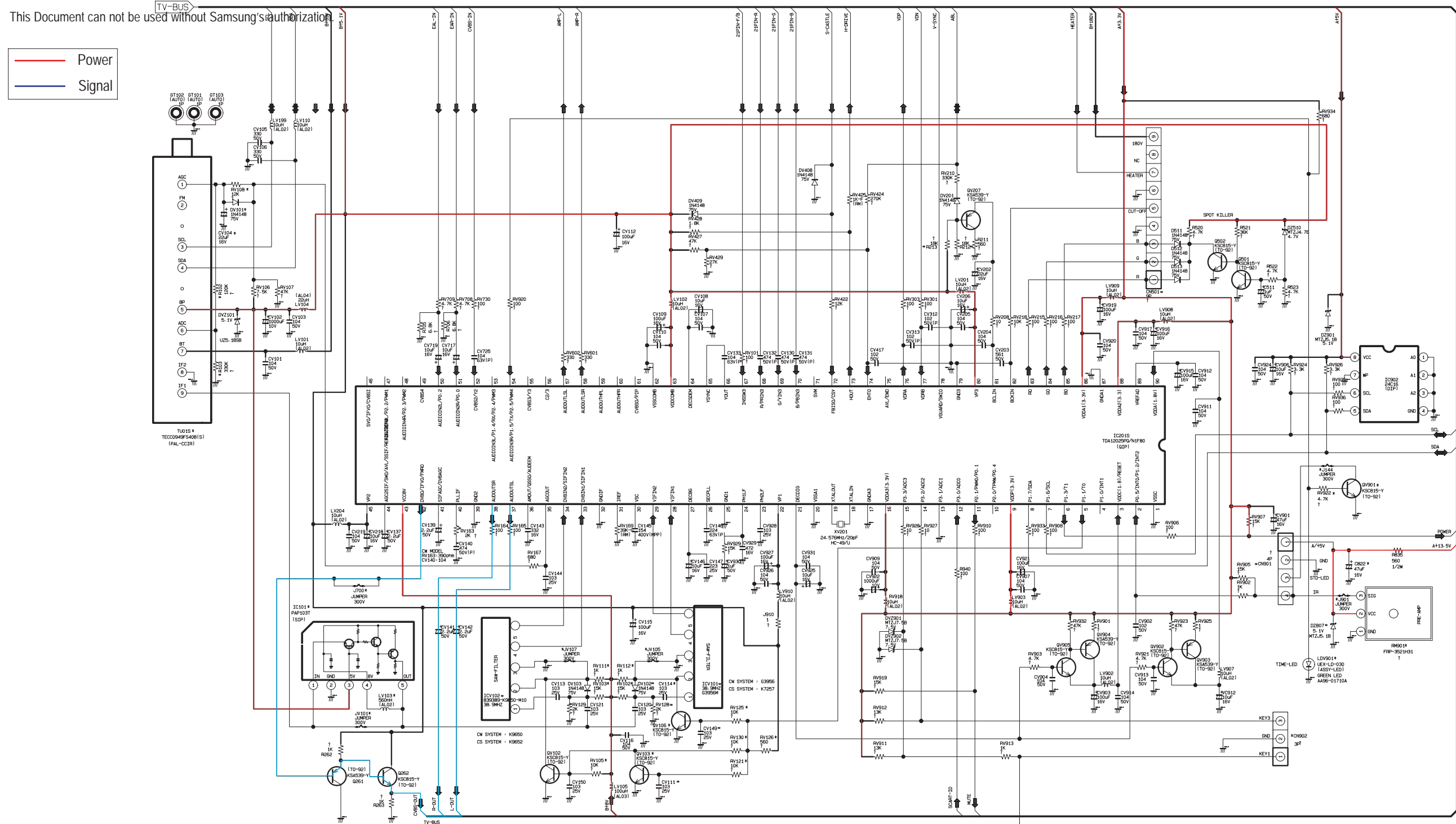
BLOCK 2 : UOC3 & TUNER BLOCK UOC3
