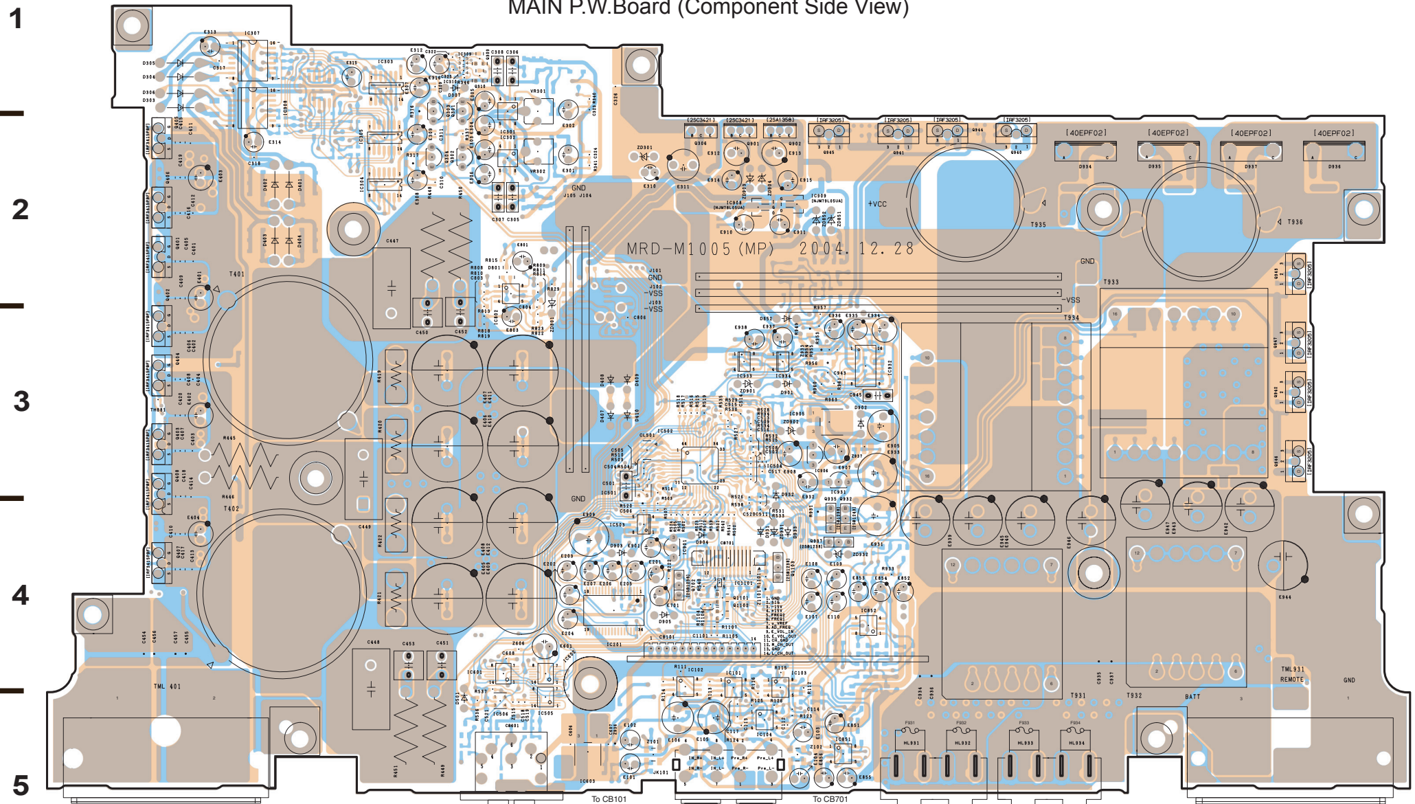
MAIN P.W.Board (Component Side View)
