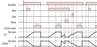
A-5 : Signal ON delay 3 (Timer resets when power comes ON.)
