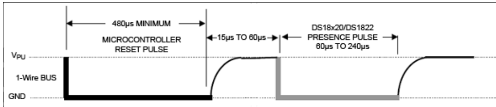
Figure 2. Reset pulse and presence pulse.
