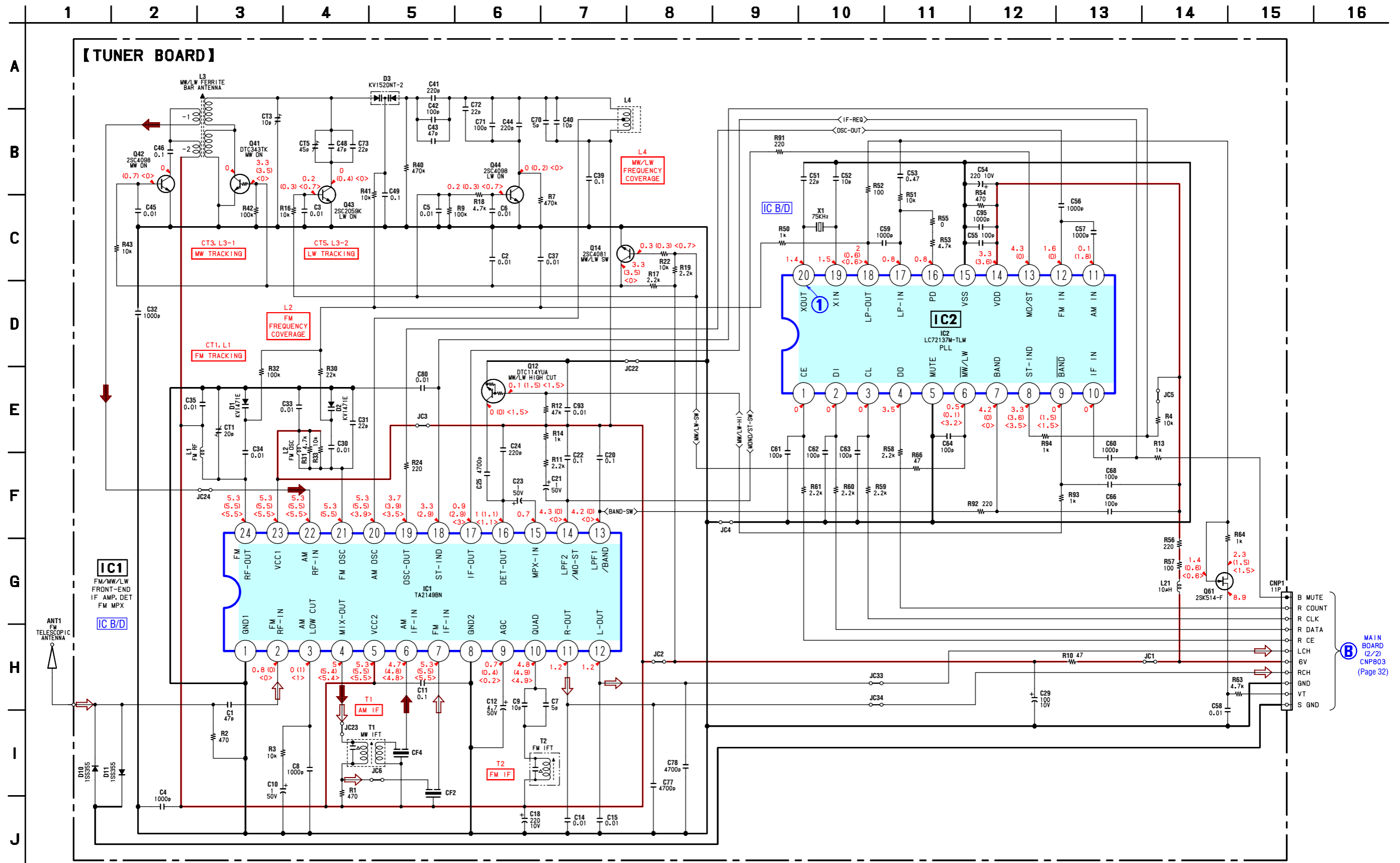
6-10. SCHEMATIC DIAGRAM – TUNER-3 BAND SECTION – • See page 41, 42 for IC Block Diagrams. • See page 39 for Waveform.
