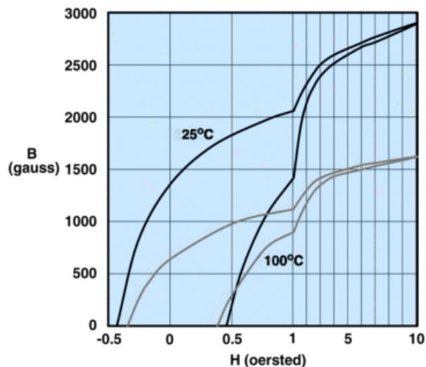
Hysteresis Loop
