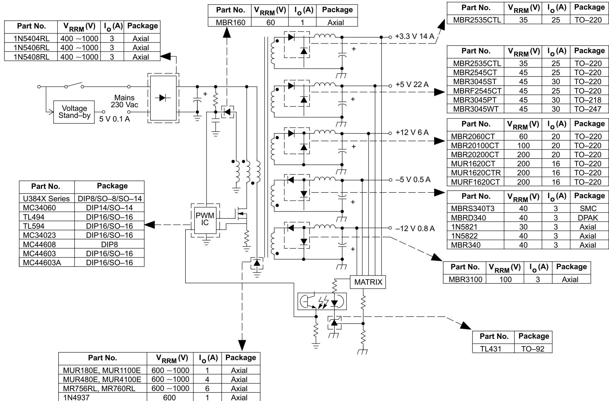
Figure 35. Typical 200 W ATX Forward Mode SMPS
