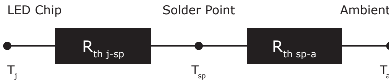
Figure 1: Thermal Resistance Model
