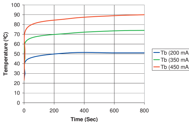
Figure 4: MCPCB Temperature
