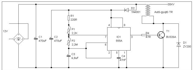
Schematic
