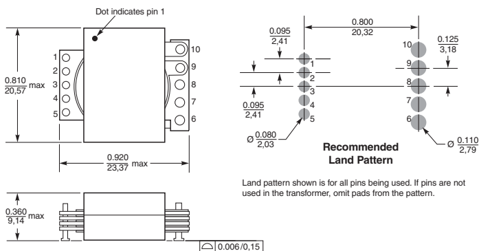
Figure 3. Typical Dimensional Drawing
