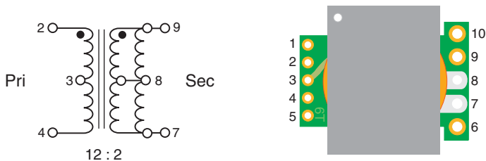
Figure 4. Sample Transformer
