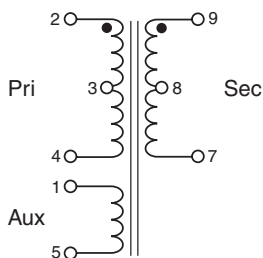
Figure 2. Typical Schematic
