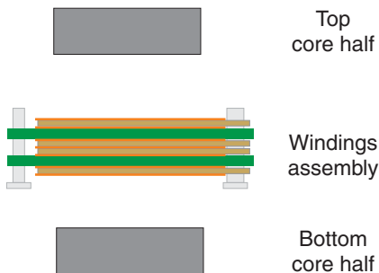
Figure 1. Major Components of a Planar Transformer
