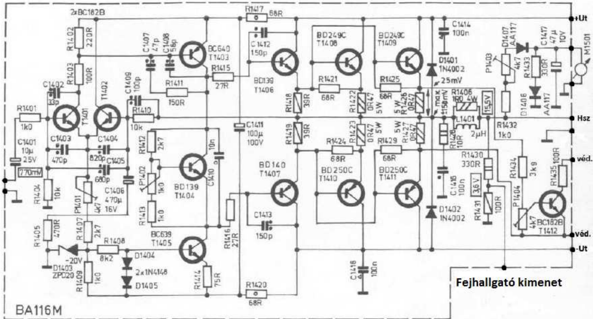
ORION SE260 amplifier Schematic
