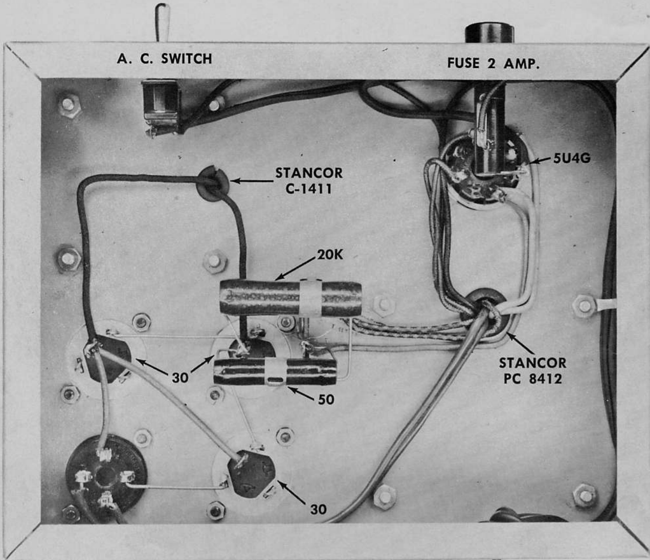
POWER SUPPLY UNIT
