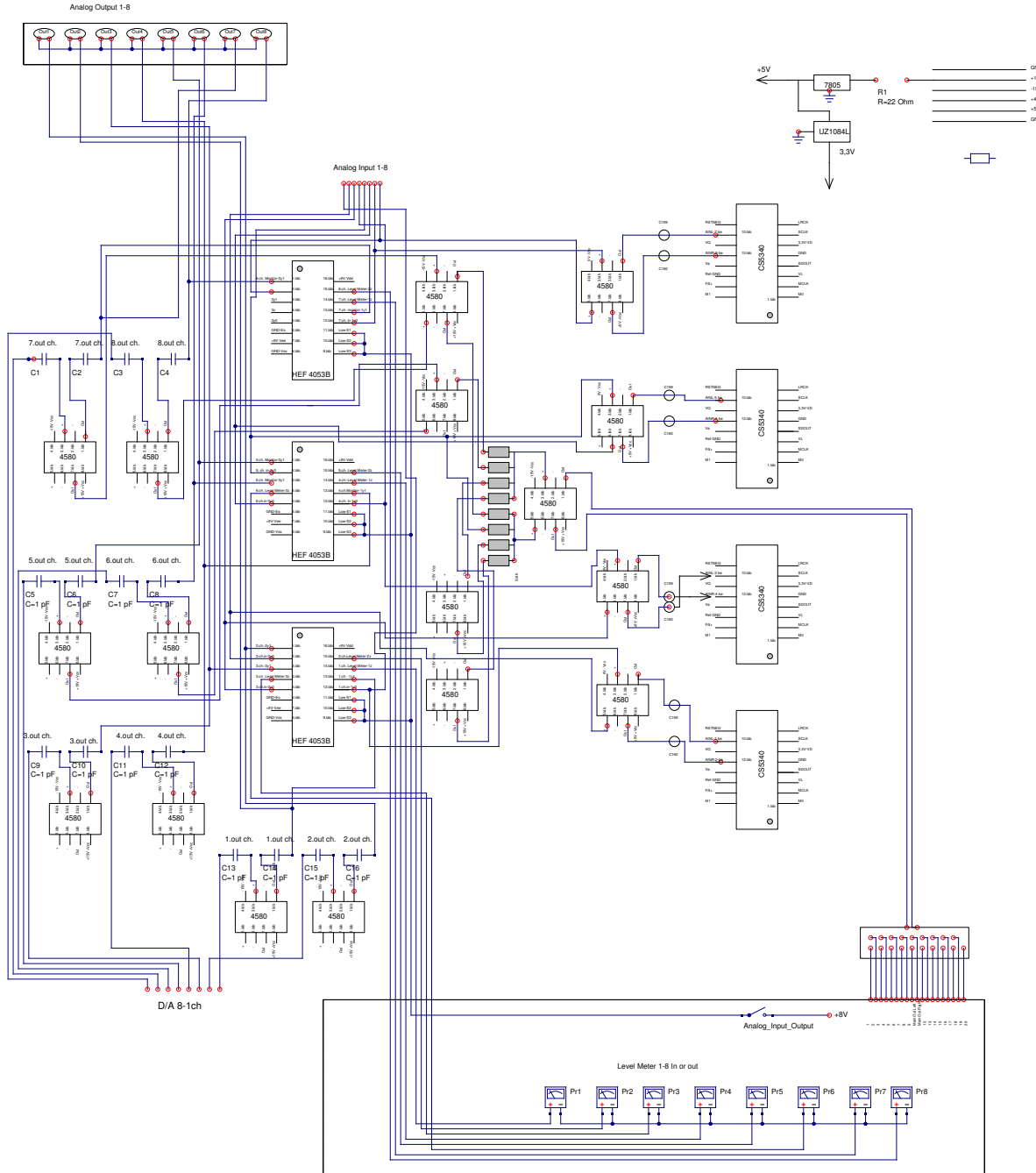
Phonics Firefly 808 block schematic
