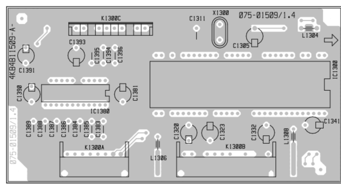
P.C.B. CIRCUITO AUDIO CARA COMPONENTES AUDIO P.C.B. COMPONENTS SIDE P.C.B. PANNELLO AUDIO LATO COMPONENTI
