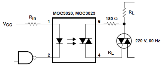
Figure 5. Resistive Load
