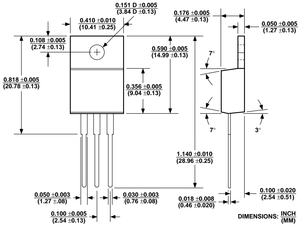
TO-220 (T)
