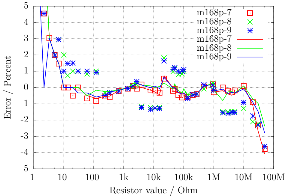
Figure 5.22. Relativ error for resistor measurements with three ATmega168P
