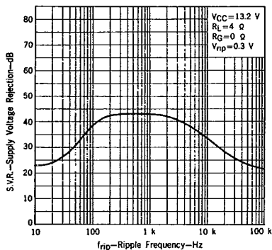
SUPPLY VOLTAGE CHARACTERISTICS
