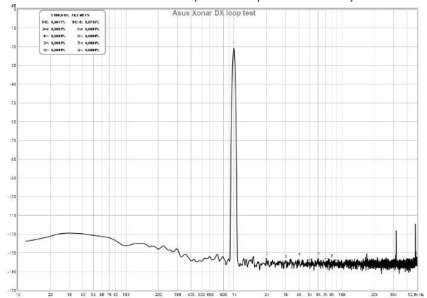
AISO 192kHz THD=0,0011%, THD+N=0,0718%
