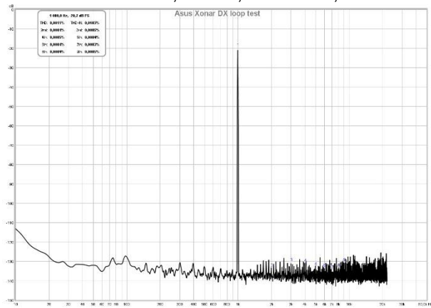
AISO 44kHz THD=0,0011%, THD+N=0,0103%
