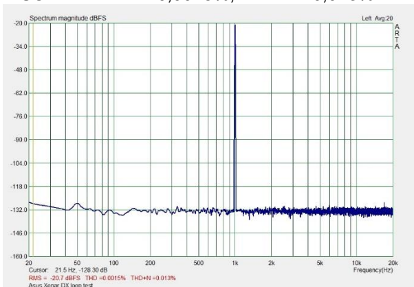
AISO 44kHz THD=0,0015%, THD+N=0,013%
