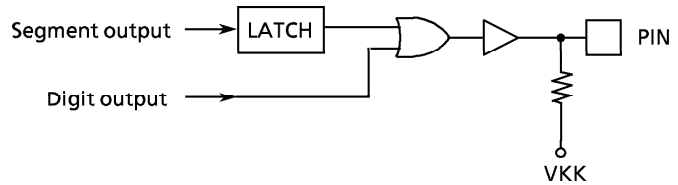
Figure 2-6. G/S port
