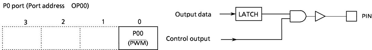
Figure 2-2. P0 port
