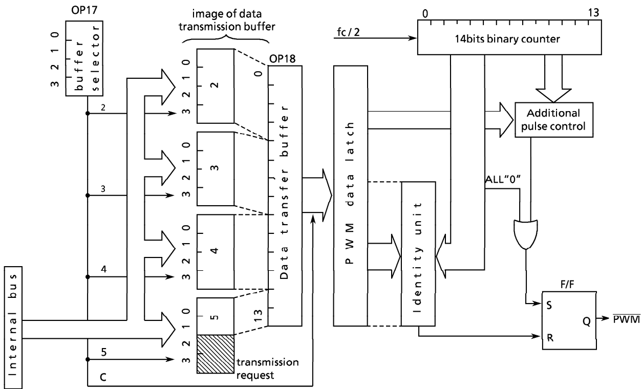
Figure 2-9. Pulse width modulation circuit
