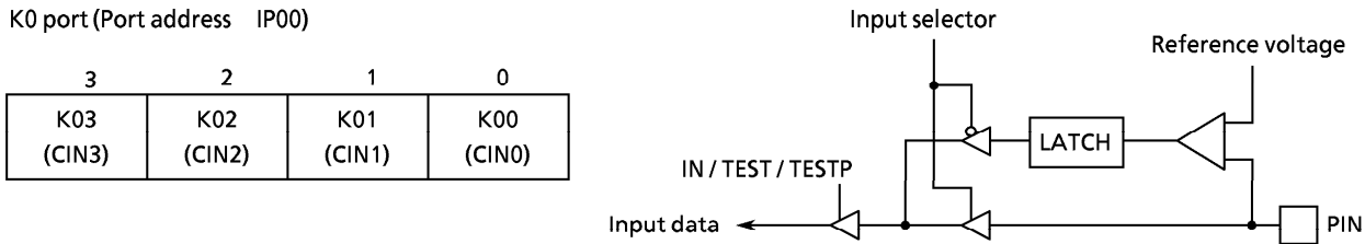
Figure 2-1. K0 port
