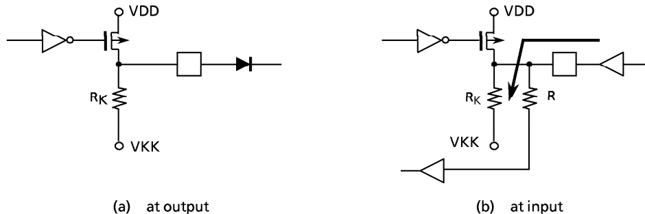
Figure 2-18. Input/Output interface
