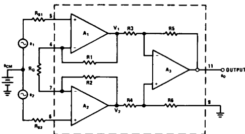
FIGURE 1. Simplified LH0036
