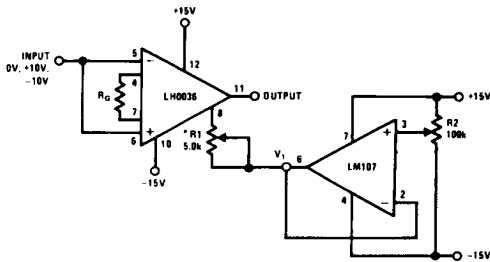
*Note: Nominal value R1 to Achieve Optimum CMRR is 3.0 k \Omega FIGURE 7. Improved V_{OS} , CMRR Nulling Circuit
