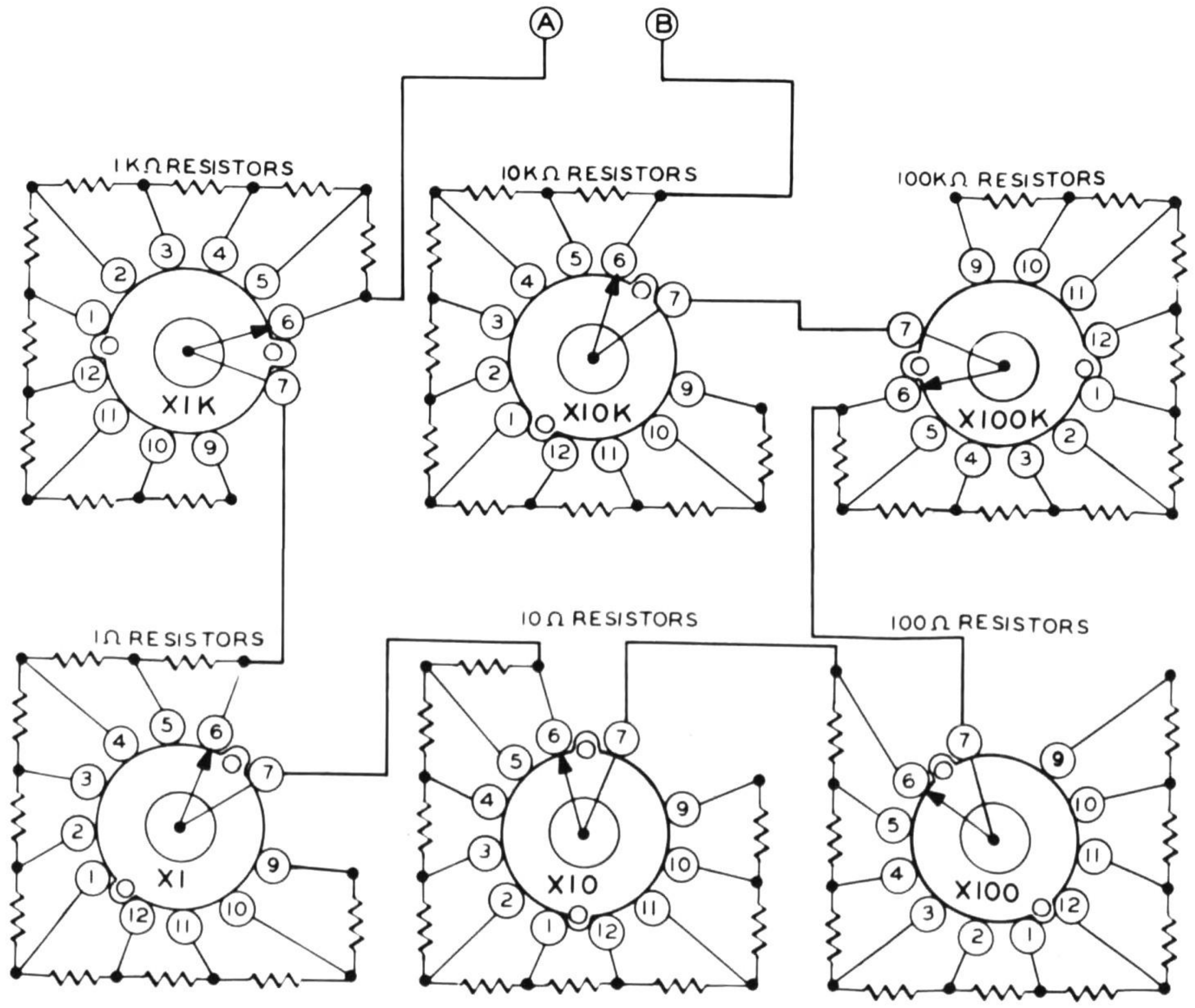
SCHEMATIC OF THE HEATHKIT® DECADE RESISTANCE KIT MODEL IN-3117
