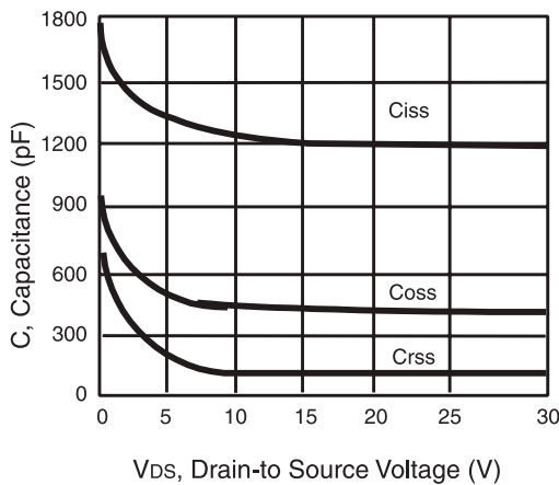
Figure 3. Capacitance
