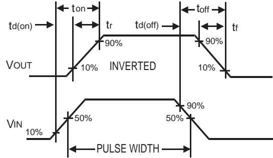
Figure 12. Switching Waveforms
