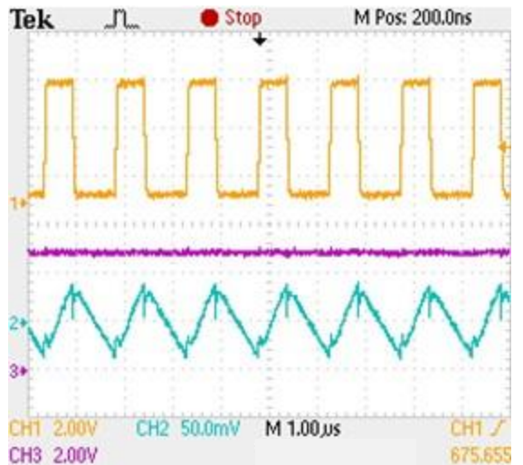
Vout=5V Vin=3V Iout = 1 A
