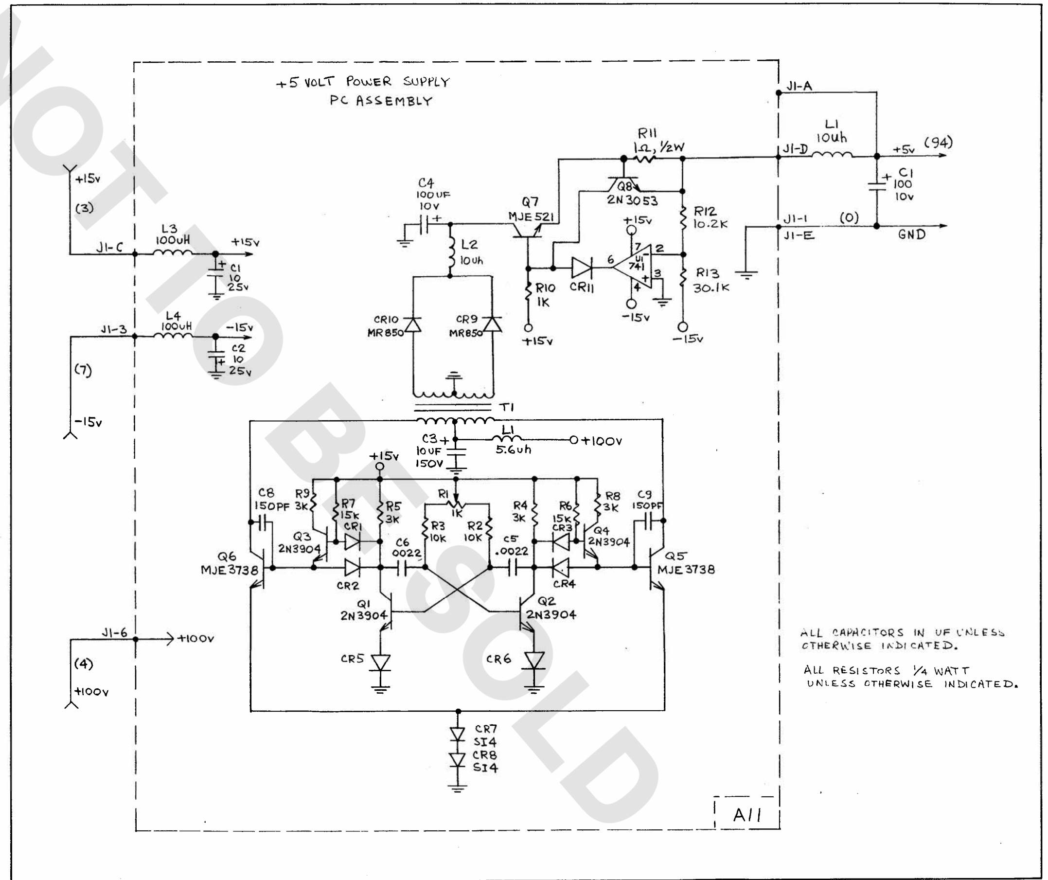
Figure 5-17. 5 Volt Power Supply
