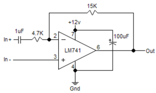
Simple preamplifier for Bose subwoofer (CE 2007)
