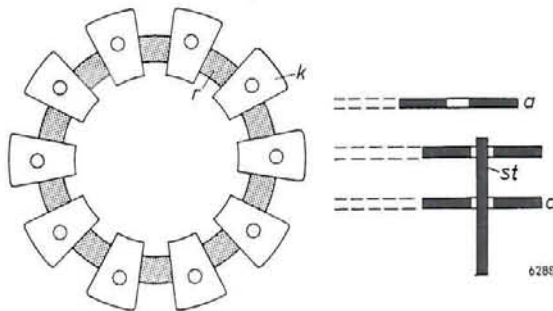
Fig. 2. Schematic representation of the electrode arrangement in the Type Z 550 M indicator tube.
