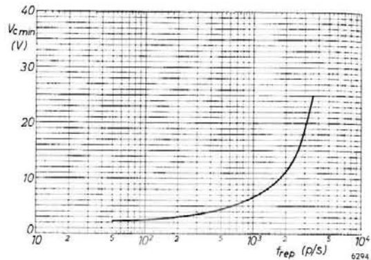
Fig. 8. Minimum required control voltage V_{c \text{ min}} as a function of the repetition frequency f_{rep} of the supply voltage.
