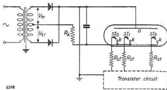
Fig. 12. Practical circuit of the indicator tube controlled by a transistorised scaler.
