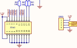
JTAG & SWD
