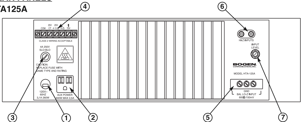
1. Power Cord: Ground Pin Connected to Chassis
