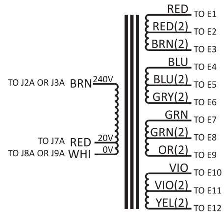
XF-000320-GP RMX1850HD, 230V
