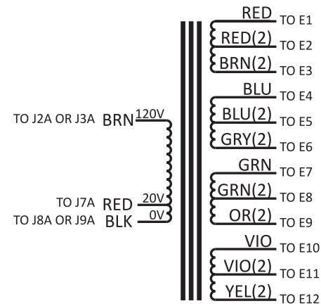
XF-000319-GP RMX2450, 120V
