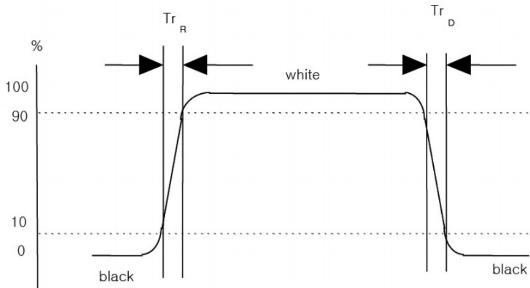
<Optical Response>
