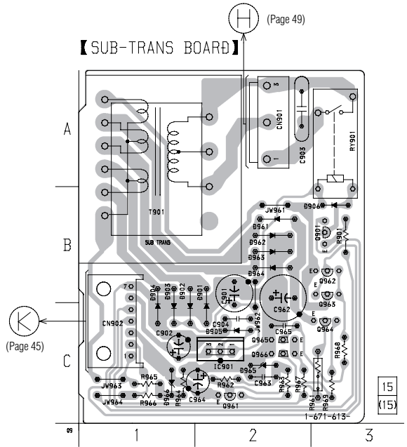
7-9. PRINTED WIRING BOARD – SUB SECTION – • See page 16 for Circuit Boards Location.
