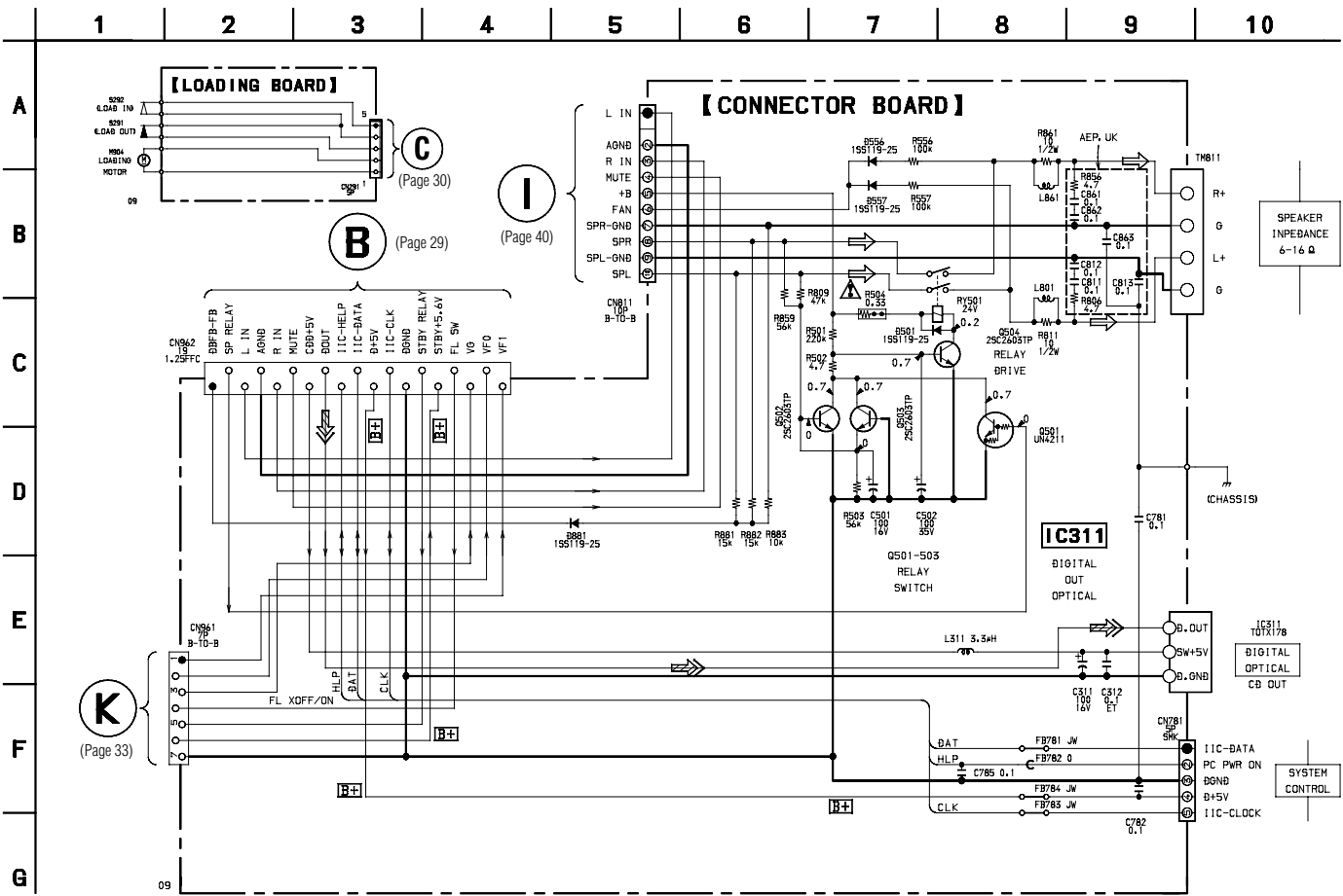
7-14. SCHEMATIC DIAGRAM - CONNECTOR SECTION -
