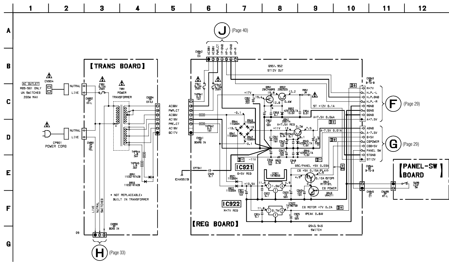
7-16. SCHEMATIC DIAGRAM – REG SECTION –
