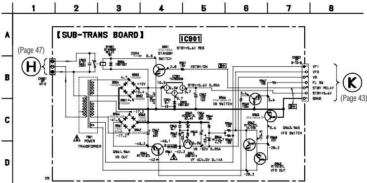
7-8. SCHEMATIC DIAGRAM – SUB SECTION –
