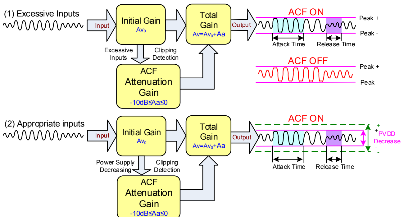
Fig. 6 the ACF Function Operation Outline
