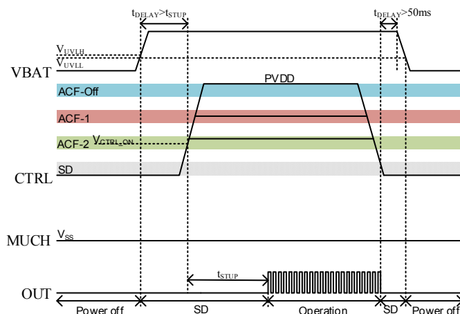
Fig. 7 Pop-Click Noise Reduction by Shutdown
