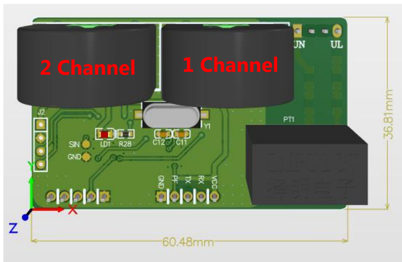
Figure 2.1 Dimensional drawing (unit: mm)
