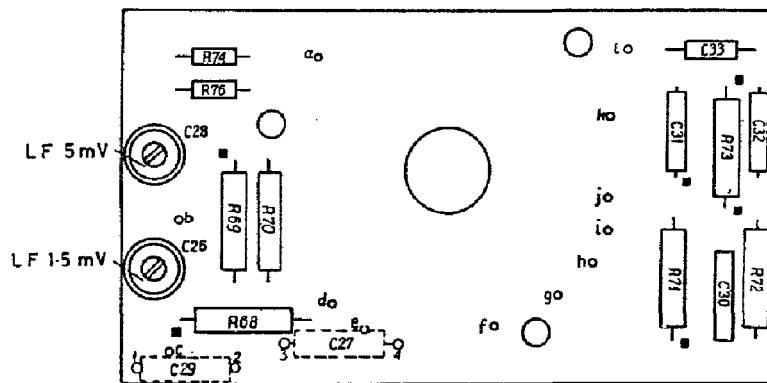
Fig 4.4 Feedback Divider (Rotary Switch) P.C.B. ( B-30-2627A )
