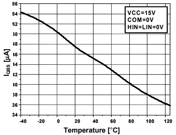
Figure 23. I_{QBS} vs. Temp.
