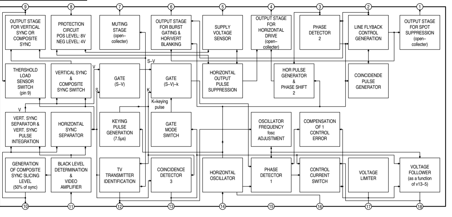
B BOARD IC301 TDA4580-V7
