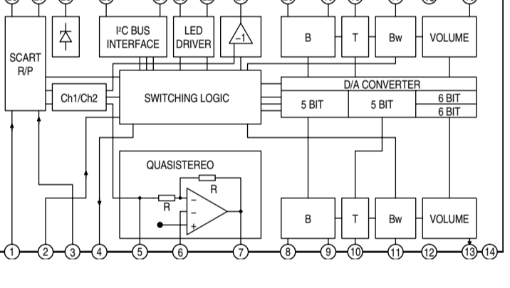
J1 BOARD IC201 TDA6200
