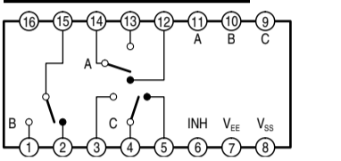
J1 BOARD IC1403 MC14053BCP
