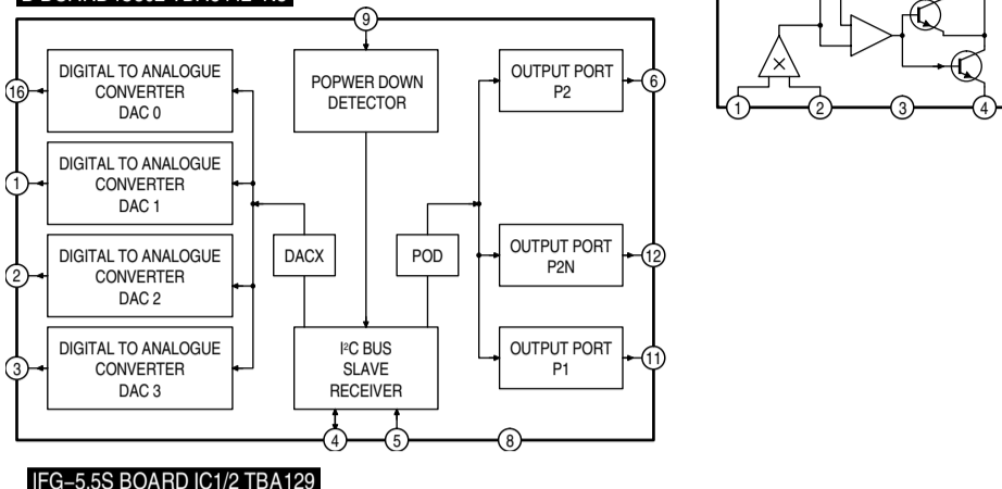
IFG-5.5S BOARD IC12 TBA129
