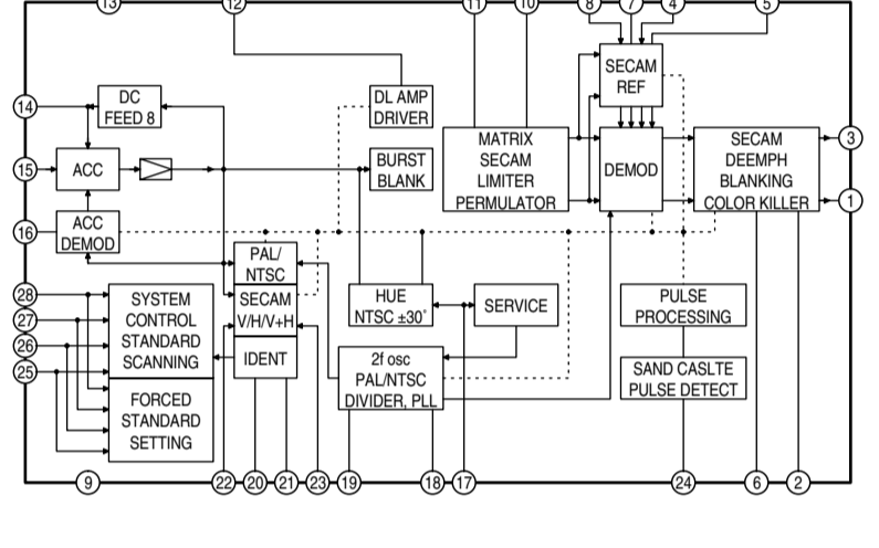
B BOARD IC331 TDA4650/V4
