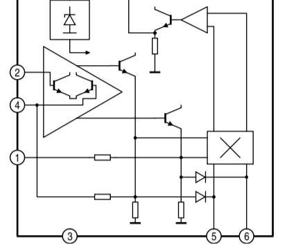
IFG-5.5S BOARD IC12 TBA129
